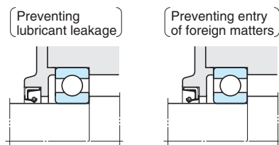
Fig. 14-9 Direction of sealing lips and their purpose
