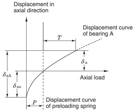
Fig. 11-2 Preloading diagram in constant pressure preloading
