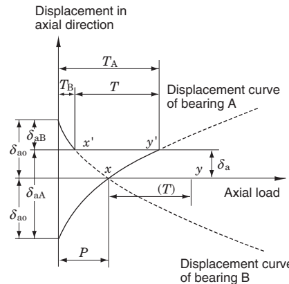
Fig. 11-1 Preloading diagram in position preloading
