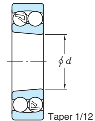
Tapered bore
