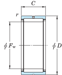
NK ( \phi F_w \geq 12 ), NKS, RNA48, RNA49, RNA69 ( \phi F_w \leq 35 )
