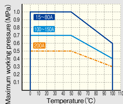
Body material : PVDF
