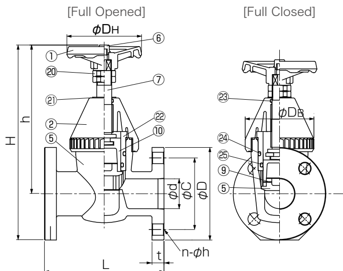
Figure (Flange Type · TS Socket Type · Thread Type)
