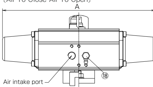
Figure (Flange Type · TS Socket Type · Thread Type · Butt Type)
