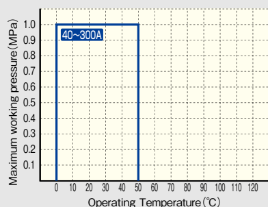
Body material : PVC
