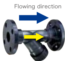
Horizontal piping
